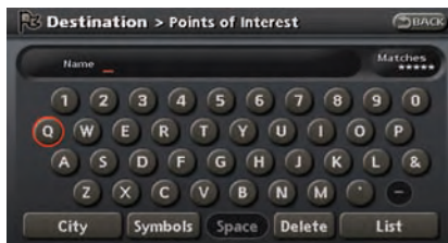
QWERTY layout
